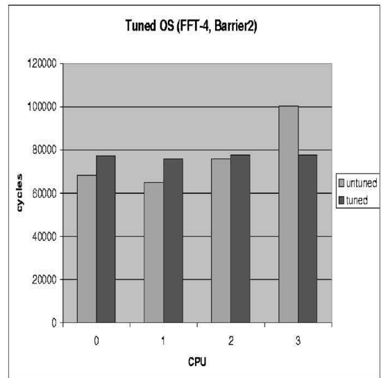
Fig. 13. Predicted impact of tuning the OS.
