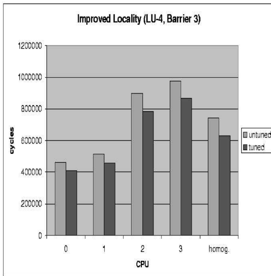
Fig. 12. Performance impact of improved memory locality.
