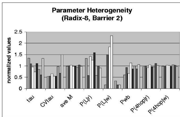
Fig. 4. Parameter heterogeneity of Radix-8, barrier 2.
