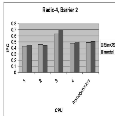
Fig. 7. Validation of Radix-4, barrier 2.
