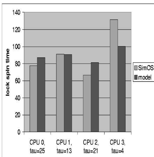
Fig. 10. Validation of processor throughput estimates with lock contention (“Sieve of Eratosthenes” algorithm on four CPUs).
