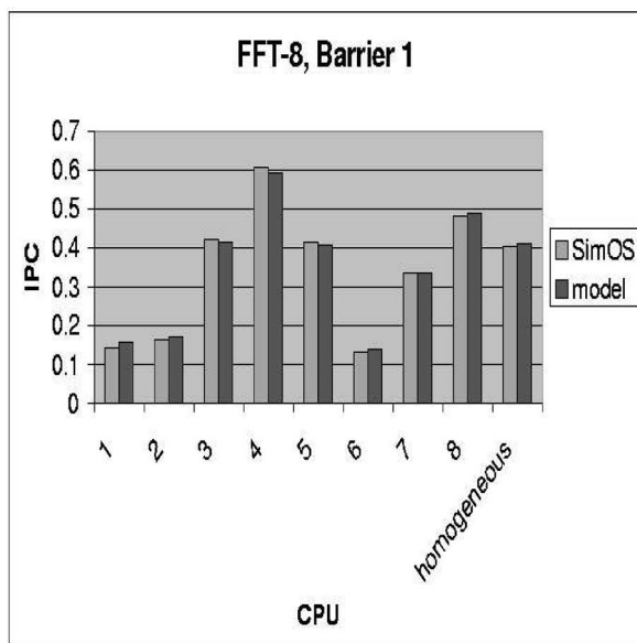
Fig. 6. Validation of FFT-8, barrier 1.
