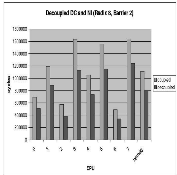
Fig. 11. Impact of decoupling DC and NI.
