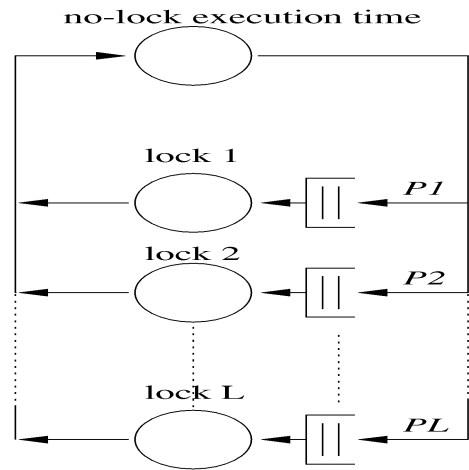
Fig. 5. Example lock contention model.
