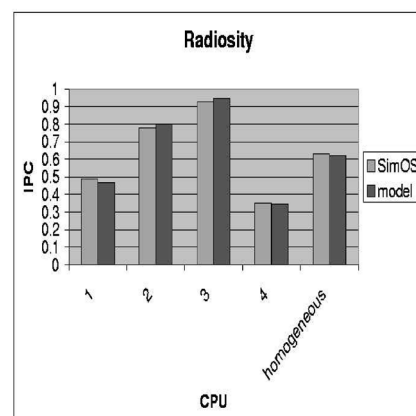
Fig. 8. Validation of Radiosity-4.
