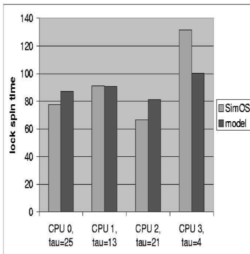
Fig. 9. Validation of lock contention estimates (“Sieve of Eratosthenes” algorithm on four CPUs).
