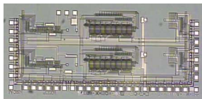
Receive Chip
