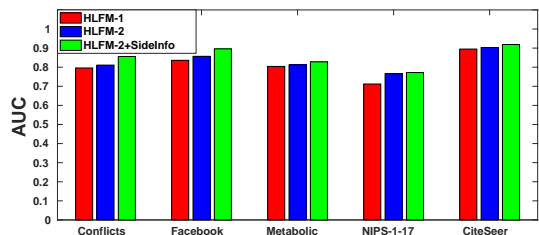
Figure 2. Comparing the three variants of our model on the data sets with side information.
