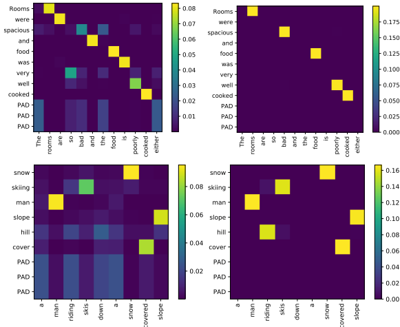
Figure 3: A comparison of OT (left column) and SEPAM (right column). The horizontal axis are the generated texts, and the vertical axis are the partial targets.
