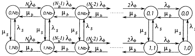
Fig. 2. Markov chain of availability model.
