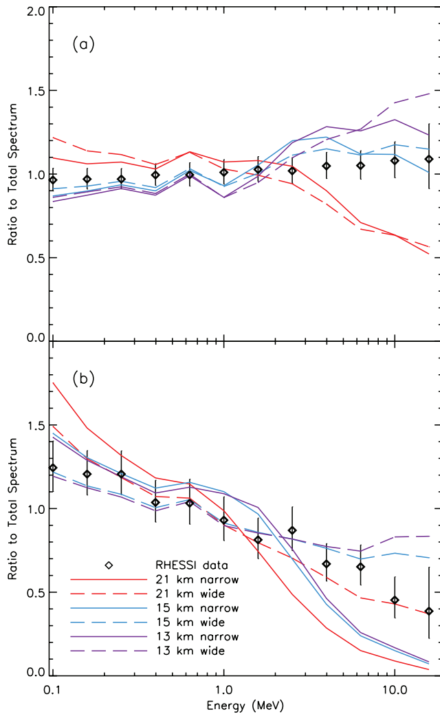
Figure 3. Data as in Figure 1, models using the random lightning flash algorithm instead of the nearest lightning flash algorithm (see text for details).
