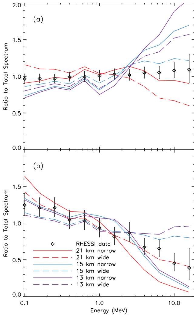
Figure 1. Ratios of the spectra of close and distant TGFs to the combined spectra of all 362 TGFs, with runaway breakdown models. (a) TGFs with close lightning flashes and models with close sources. (b) TGFs with only distant lightning flashes and models with distant sources.
