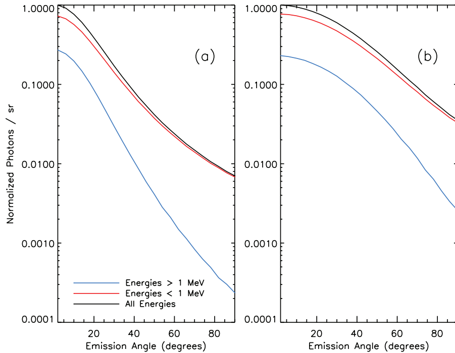
Figure 2. (a) Intrinsic beam shape from relativistic runaway simulations. Note the energy structure of the beam, with the high energy photons concentrated in a narrower emission cone than the low energy photons. (b) Wide beam shape from the convolution of the intrinsic beam shape with a gaussian in solid angle.
